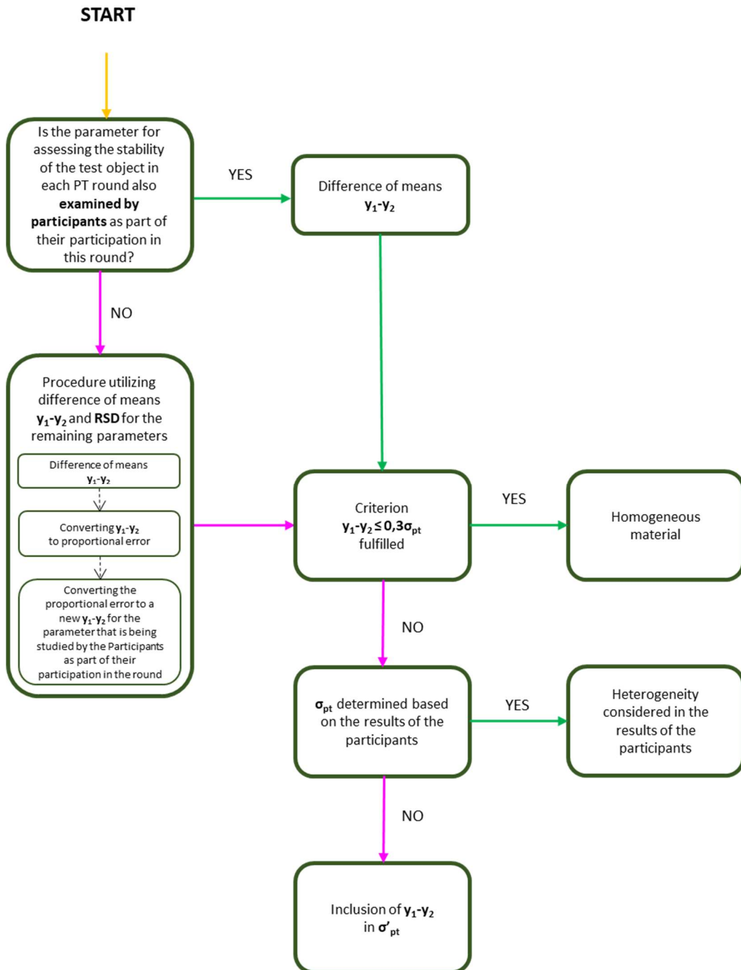
Fig. 2. Algorithm for assessing stability in proficiency testing
