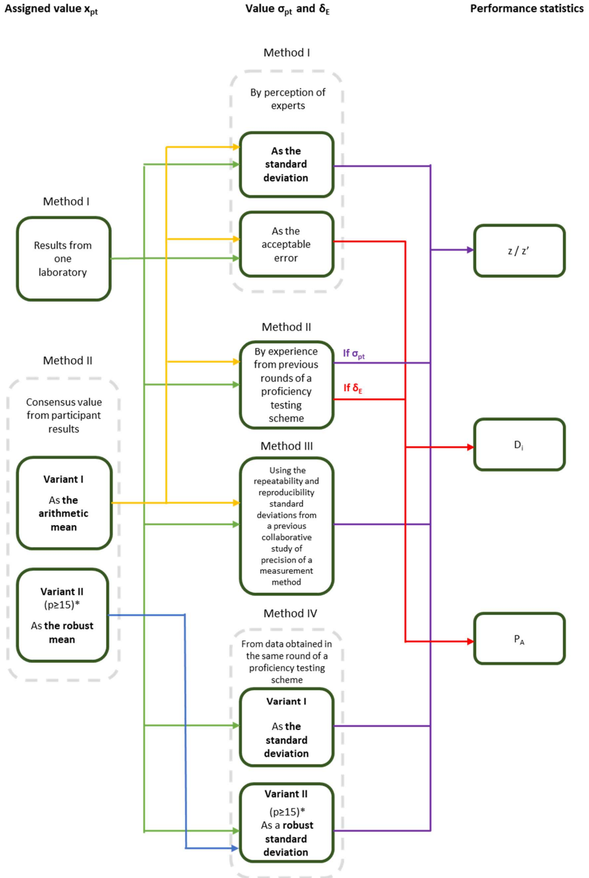
Fig. 3. Statistical model algorithm in proficiency testing
