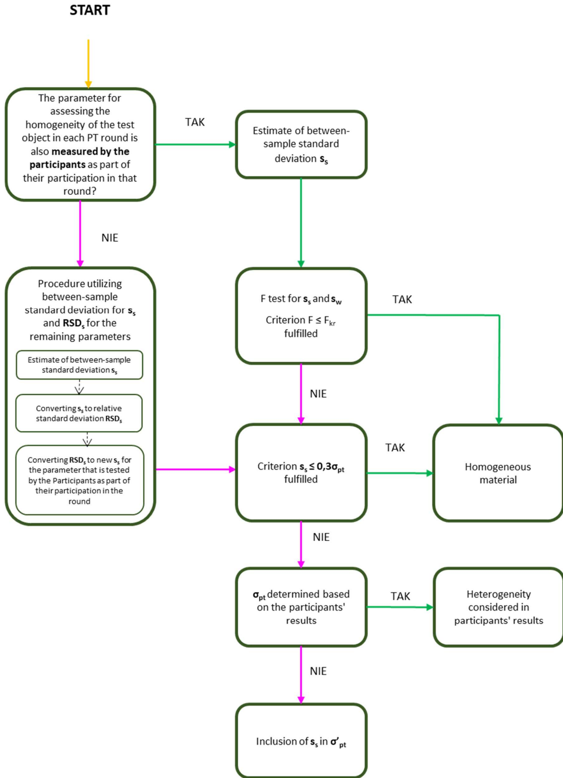
Fig. 1. Homogeneity assessment algorithm in proficiency testing
